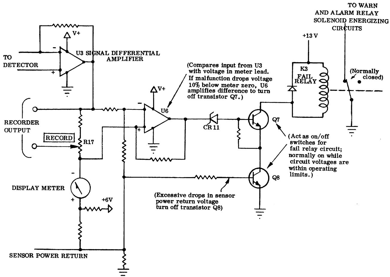
Figure 1-12. Fail Circuit Schematic Diagram
