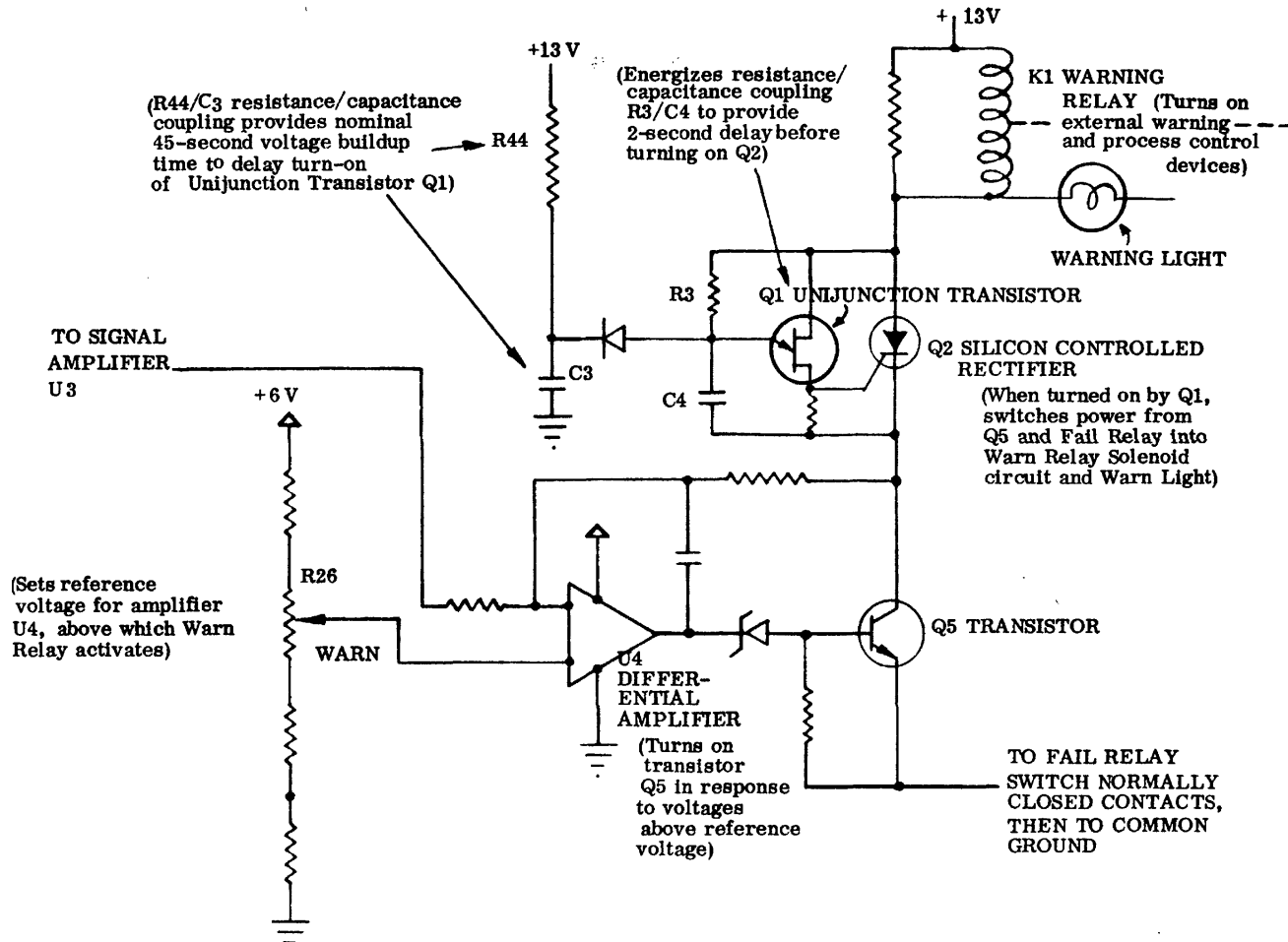
Figure 1-10. CD800/830 Warning Circuitry Schematic Diagram (typical also for Alarm circuitry)
