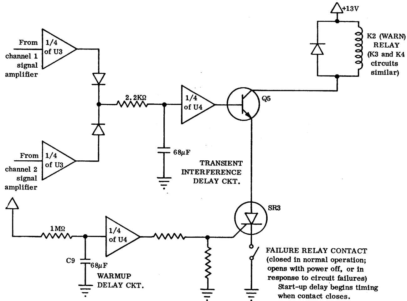
Figure 1-11. Time Delay Circuit CD802/832 Schematic Diagram
