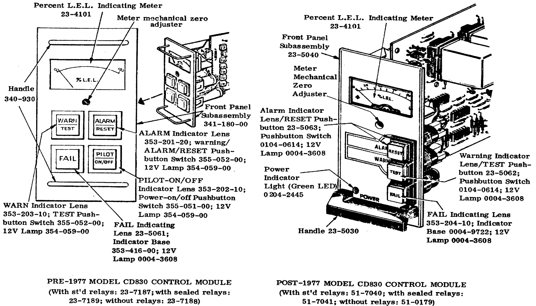
Figure 5-1. Pre-1977/post 1977 Models: CD830 Control Module Front Panel Parts Comparison
