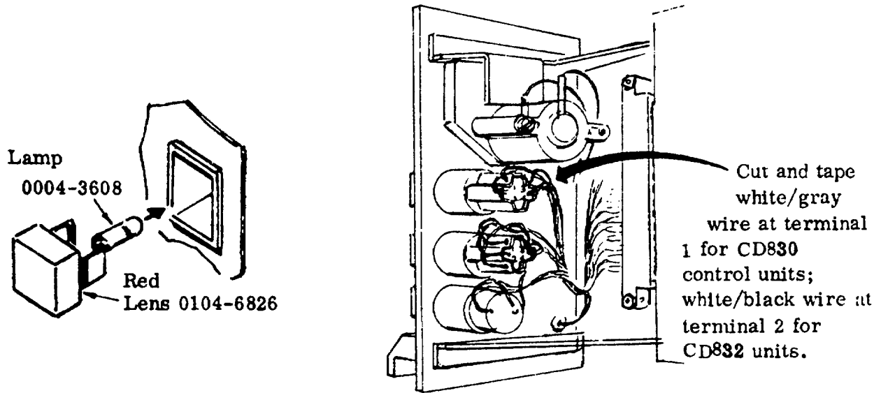
Figure 2-26. Lamp Lens Replacement, CD830/832
