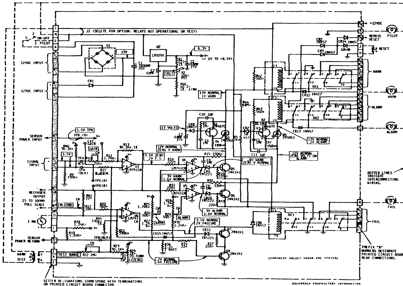
Figure 1-4. CD800/830 Printed Circuit Board Schematic Diagram
