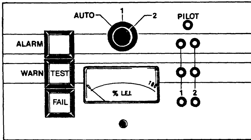
CD802W (Dual Channel) Front Panel Configuration
