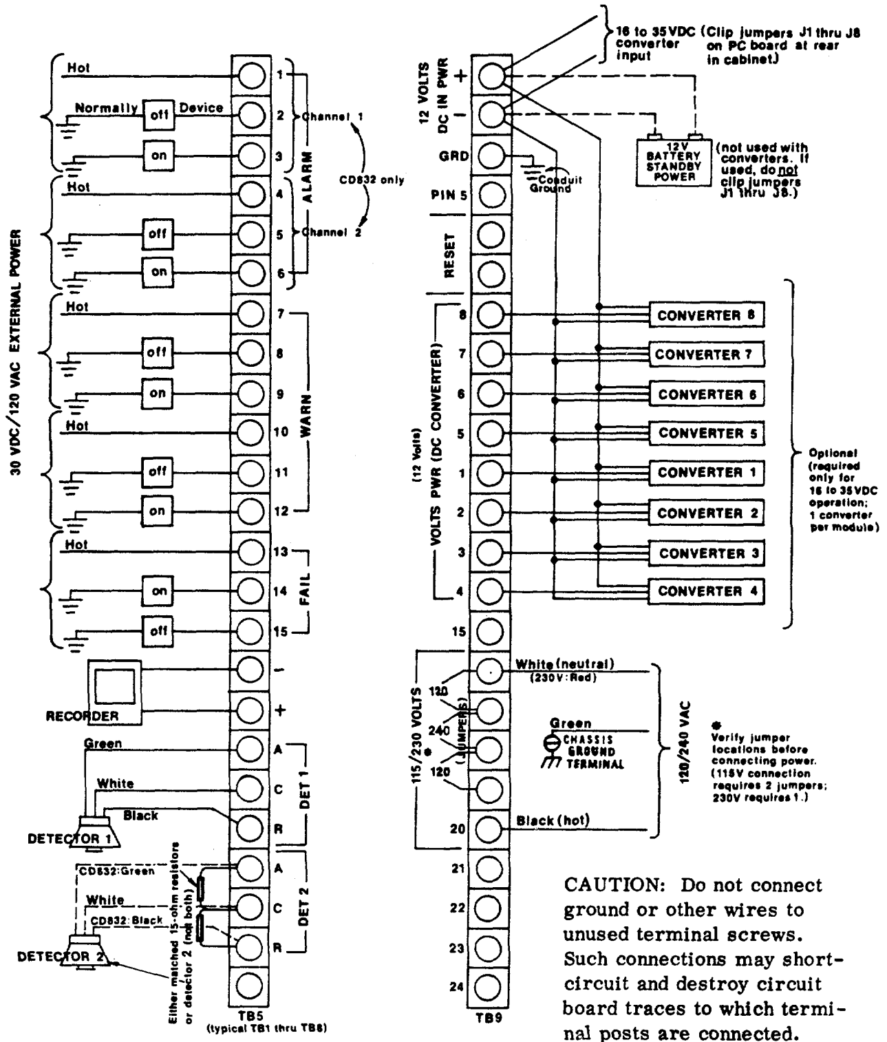
Figure 2-14. CD830W4/CD830W8 and CD832W4/CD832W8 External Wiring Connections Diagram
