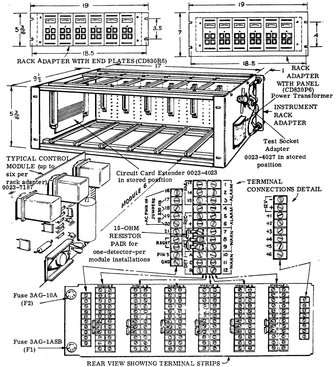
Figure 2-8. CD830 and CD832 Standard Instrument Rack Adapter for Up to Six Control Modules
