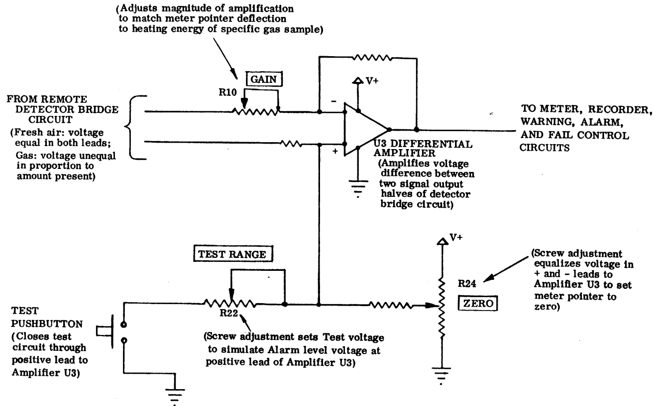
Figure 1-9. CD800/830 Signal Amplifier and Test Circuits (typical for CD802/832 circuitry also)
